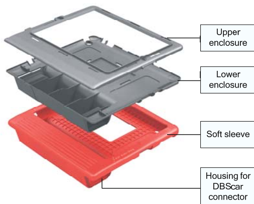
Fig. 1-3 X-431 PRO protection sleeve
