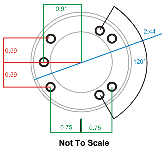
Figure 37 RAM Assembly Footprint
